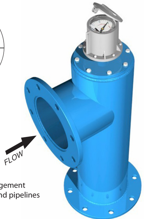
FlowCom register
