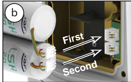
Figure 7. Non-rechargeable batteries
