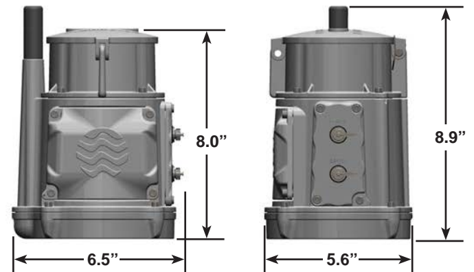
Figure 18. FlowConnect unit with non-rechargeable batteries and satellite antenna
