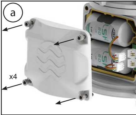
Figure 7. Non-rechargeable batteries
