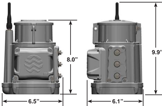
Figure 17. FlowConnect unit with rechargeable batteries and cellular antenna
