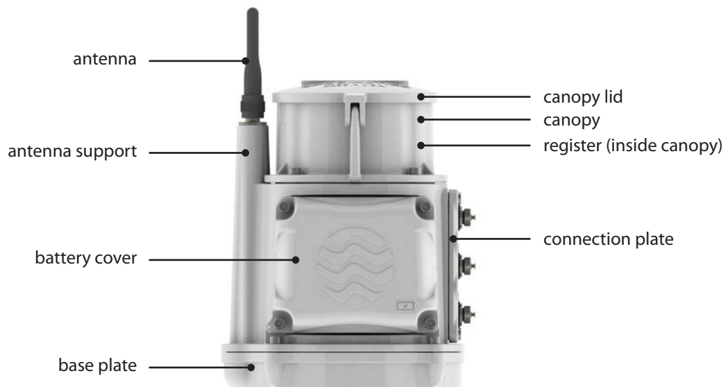
Figure 2. Accessible components
