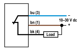
4-pin M12 Male QD
