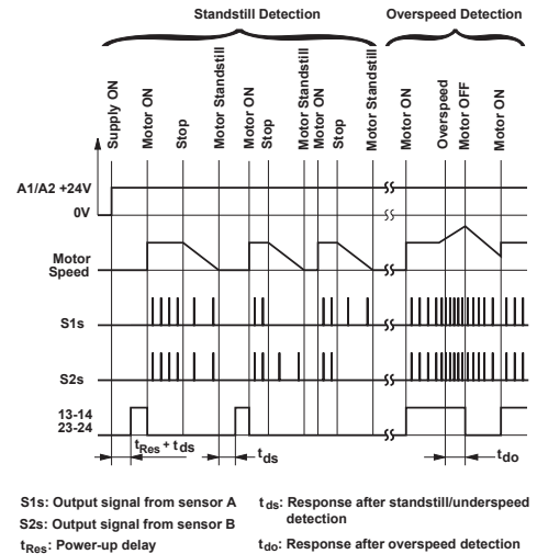
Figure 2. Functional Diagram
