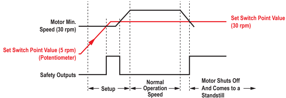
Figure 8. Under-speed Timing
