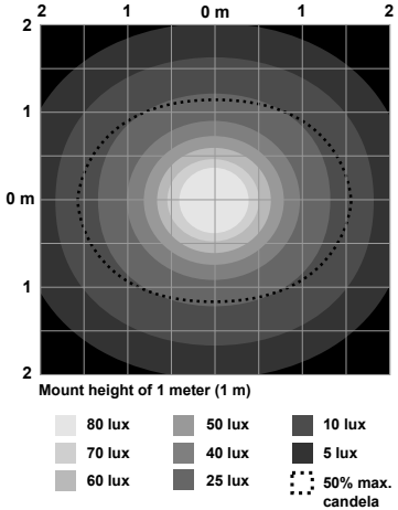
Isolux Pattern
