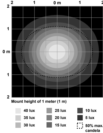
Isolux Pattern
