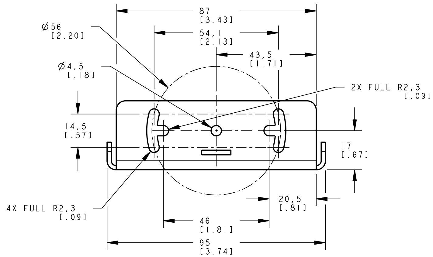
VIEW Z-Z
