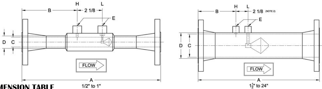
DIMENSION TABLE
