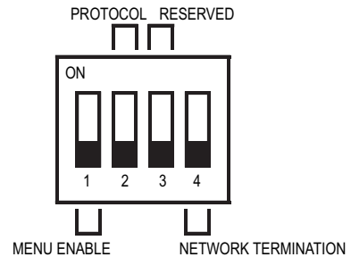
Figure 5: Dip switch SW1 (bottom-center)
