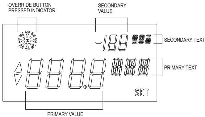
Figure 7: Display layout
